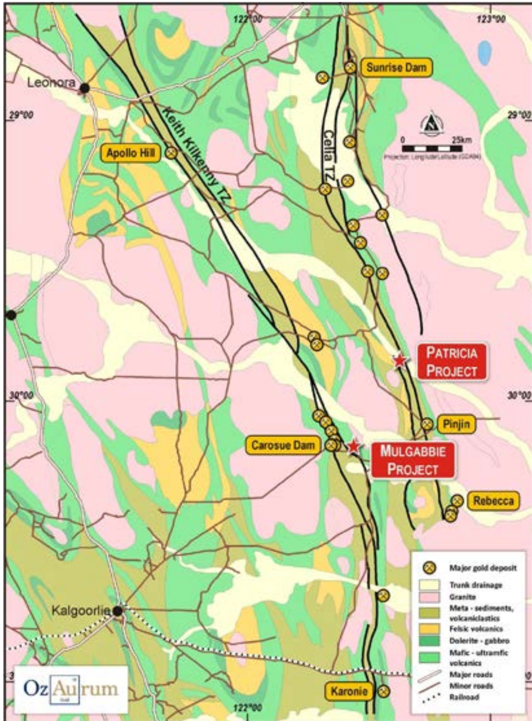
Figure 2: Geological Setting of OzAurum Projects; Polygons from GSWA 500k bedrock interpretation
